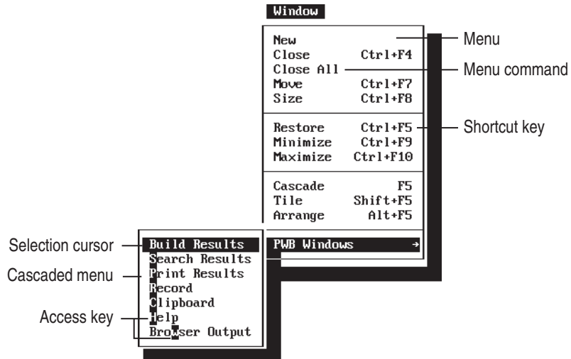
Figure 4.4 PWB Menu Elements
