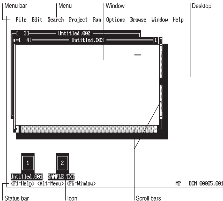
Figure 4.1 User Interface Elements
