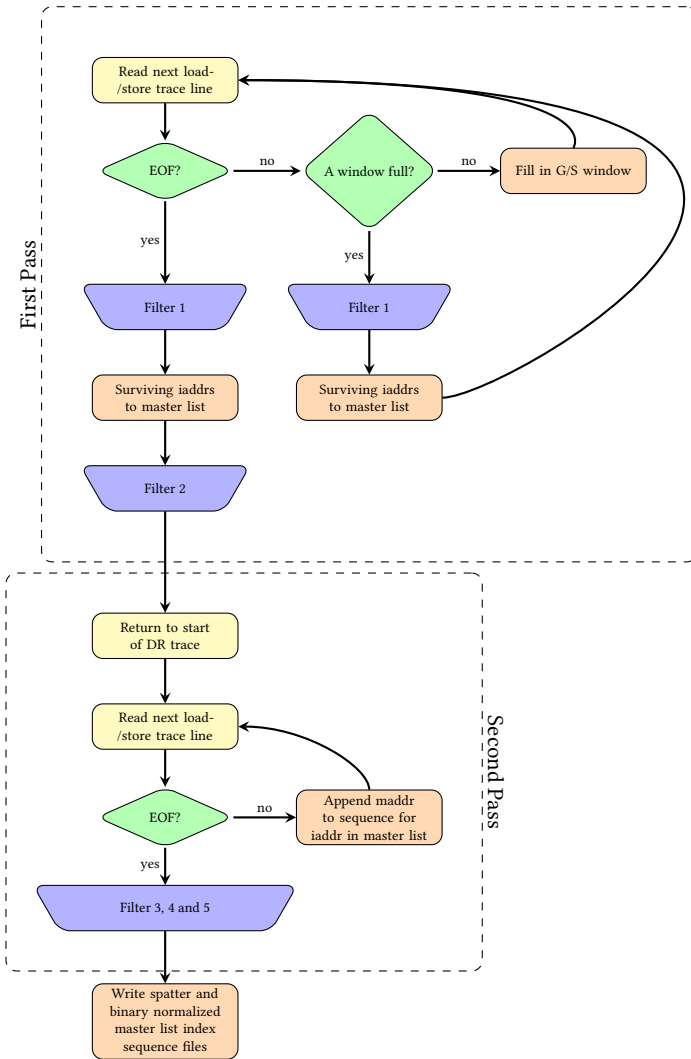
Figure 3: Core GS patterns algorithm.
