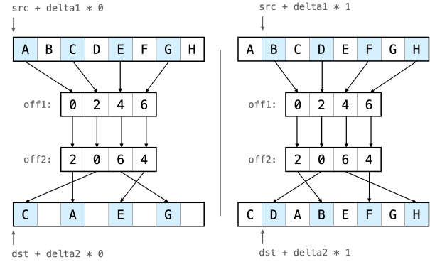
Figure 5: A visual representation of the first two iterations of the GatherScatter kernel. Both \delta_1 and \delta_2 are set to 1, and the offset buffers are shown in the figure.
