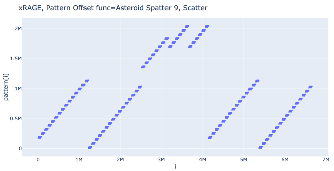
(b) xRAGE Spatter 9 scatter visualization.
