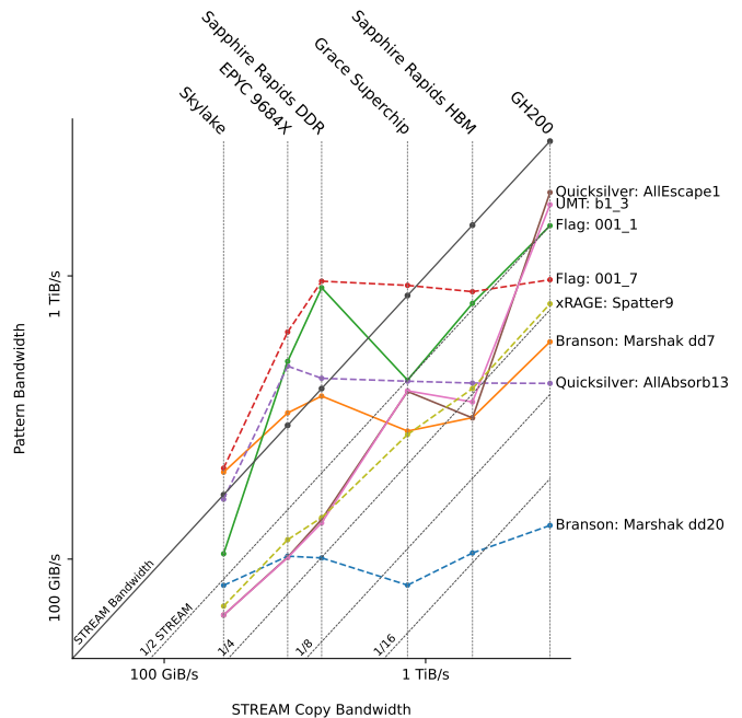
(b) CPU platform bandwidth-bandwidth plot.
