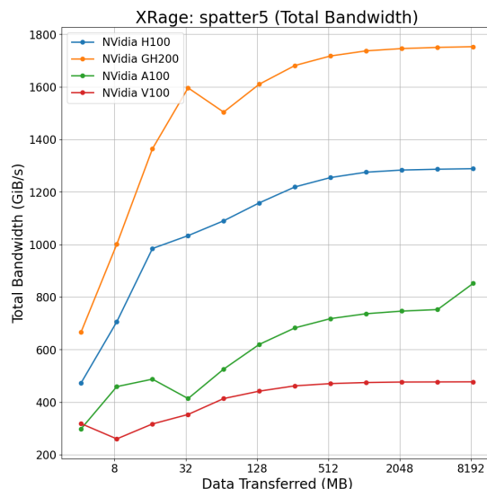
Figure 13: Spatter results across multiple generations of NVidia GPUs for an xRAGE gather pattern.
