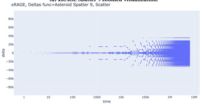
(f) xRAGE Spatter 9 deltas visualization.
