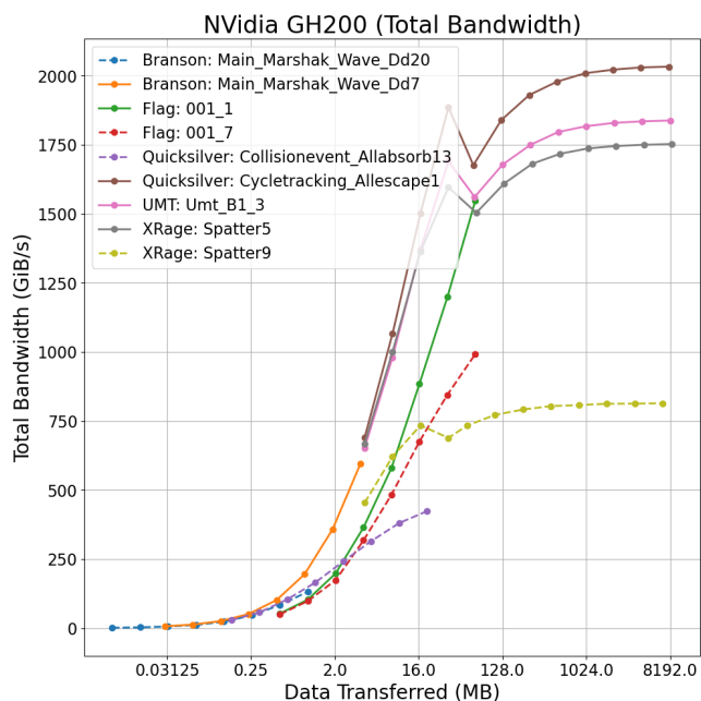
Figure 14: Spatter results of all 5 applications on GH200 GPU.
