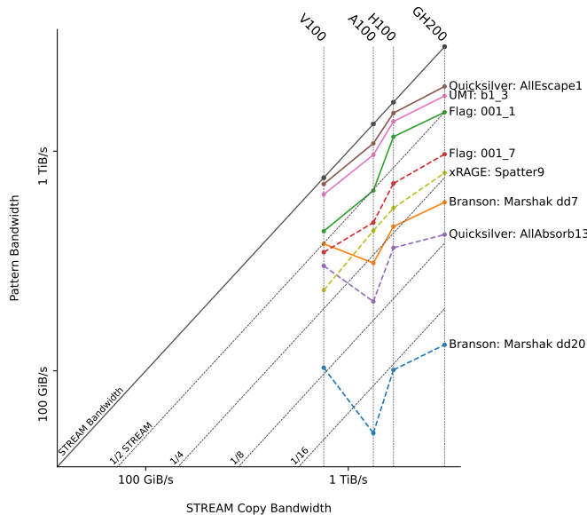
(a) GPU platform bandwidth-bandwidth plot.
