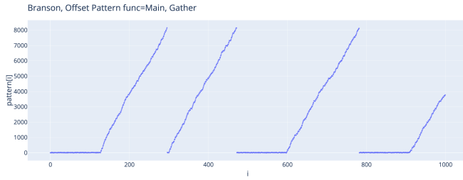
(a) Branson Gather0 Offsets
